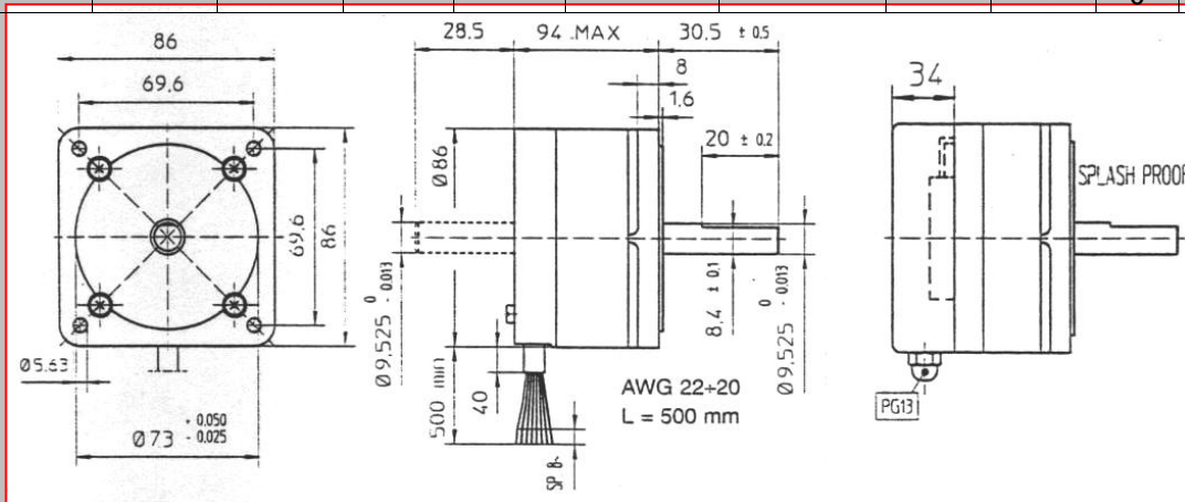
Dimensions (mm)
