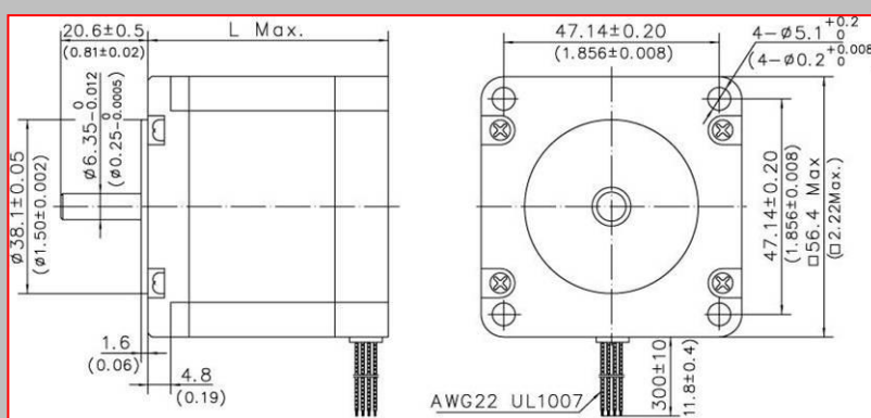
Dimensions (mm)
