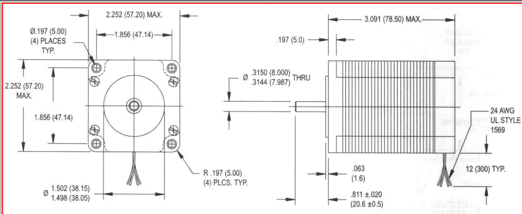
Dimensions (mm)
